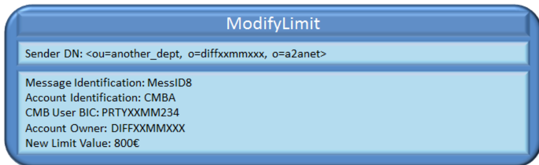
Figure 241 – Unsuccessful decrease of a CMB Limit: ModifyLimit
