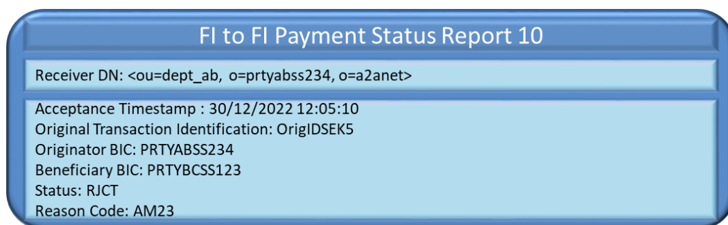
Figure 82 – Headroom error: FIttoFIPaymentStatusReport
