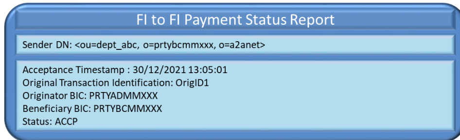
Figure 41 – Successful Instant Payment transaction: FItoFIPaymentStatusReport
