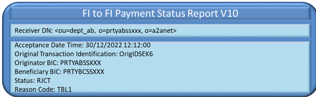
Figure 85 – Blocked account error: FItoFIPaymentStatusReport
