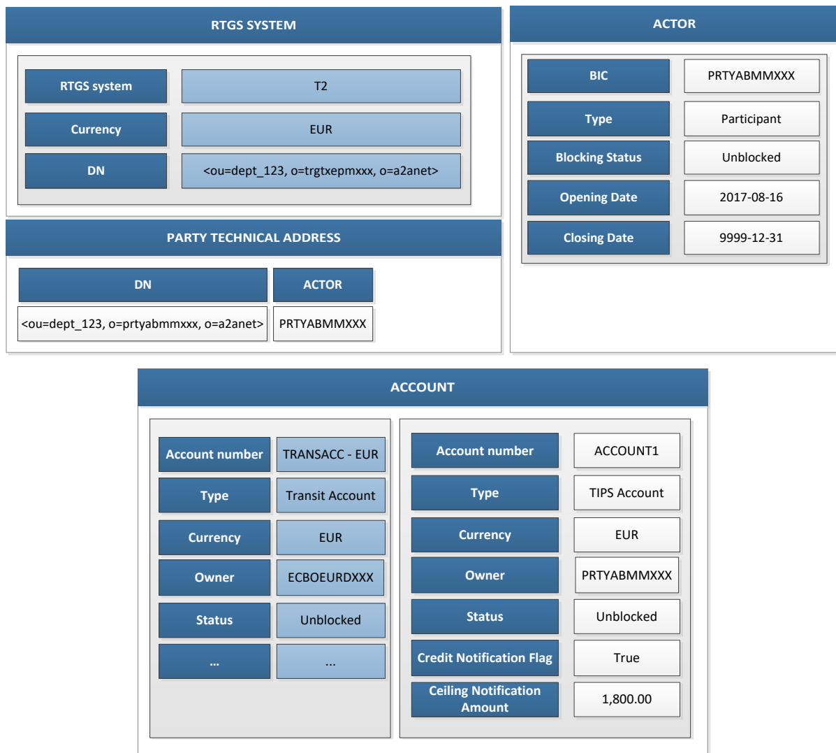
Figure 145 – Inbound Liquidity Transfer Order examples: data constellation
