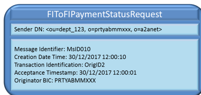
Figure 140 – Unsuccessful FIToFIPaymentStatusRequest
