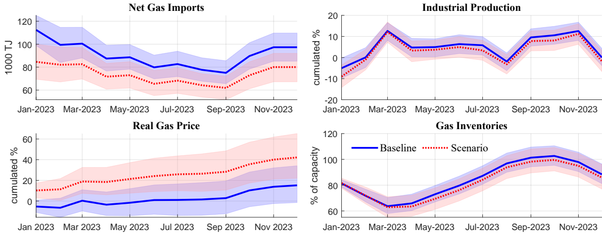
Figure 7: Conditional forecasts for a disruption of Europe I and II in January 2023
