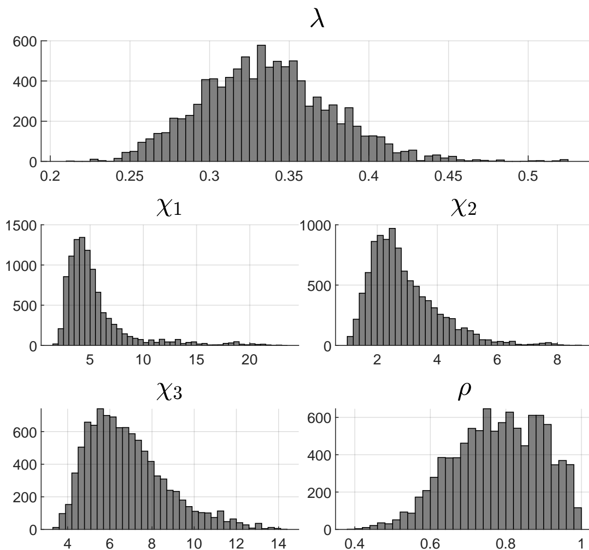
Figure A.5: Posterior distribution of the hyperparameters
