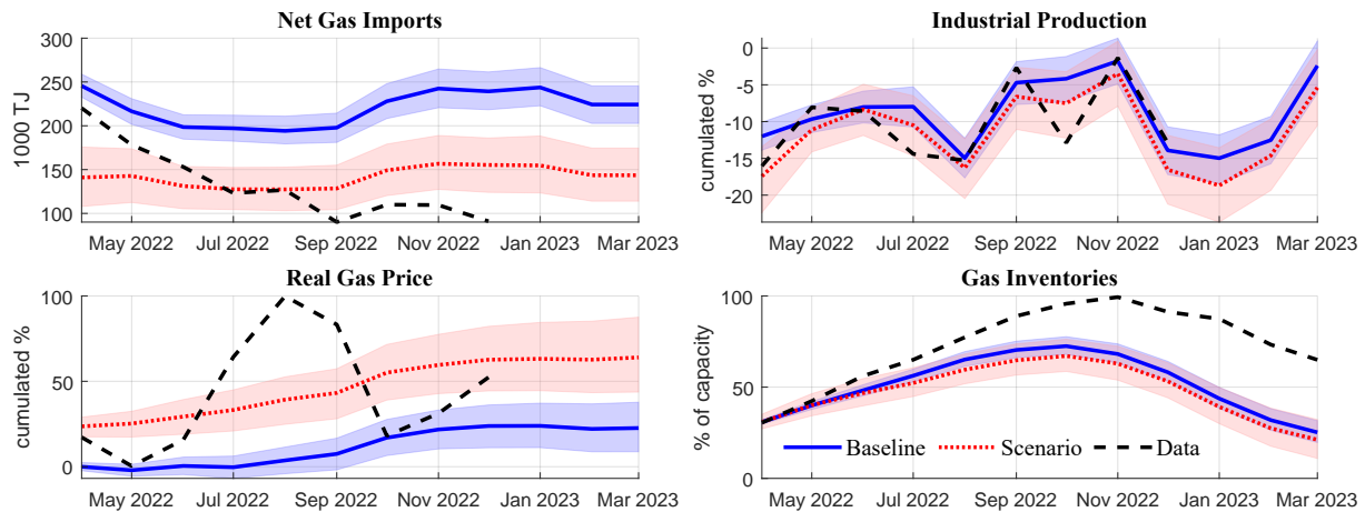
Figure 5: Conditional forecasts for a natural gas embargo against Russia starting in April 2022
