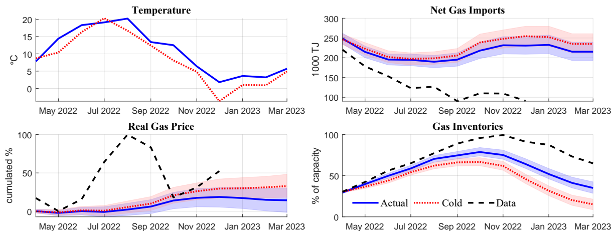
Figure 6: Conditional forecasts for actual monthly temperatures in April 2022–March 2023 and the coldest year in the sample period, April 2010–March 2011
