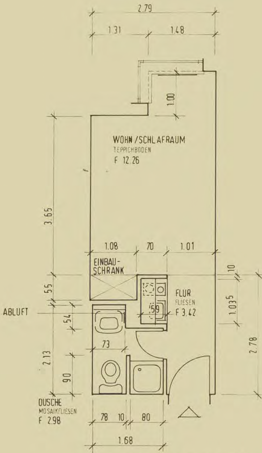
GRUNDRISS APP. 130, ■ 330
