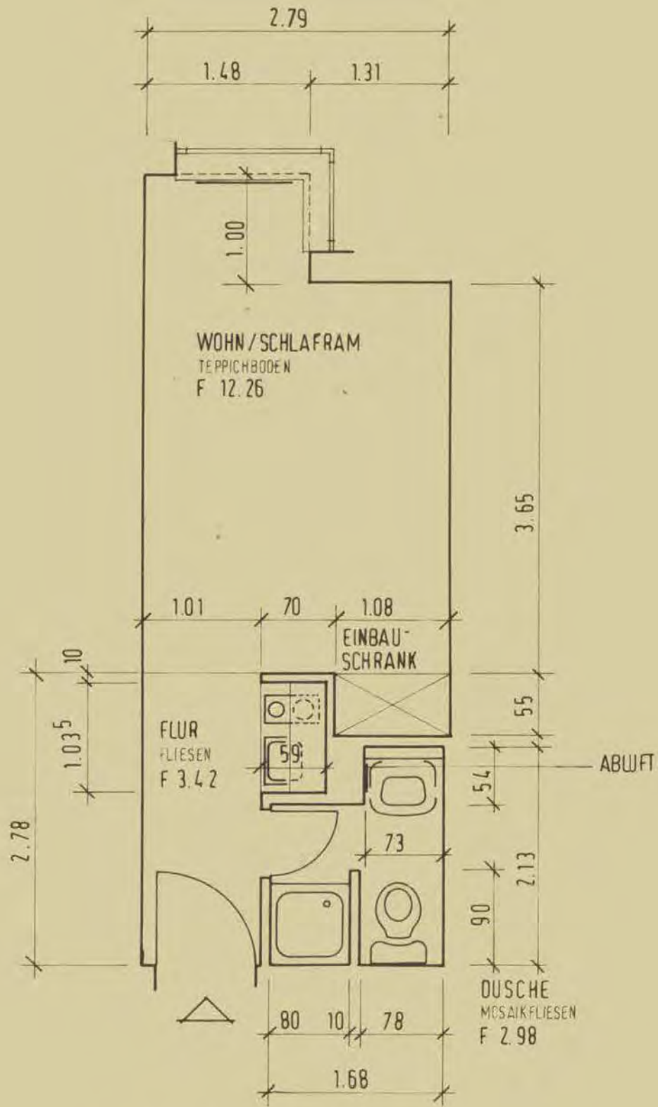
GRUNDRISS APP. 131+133
