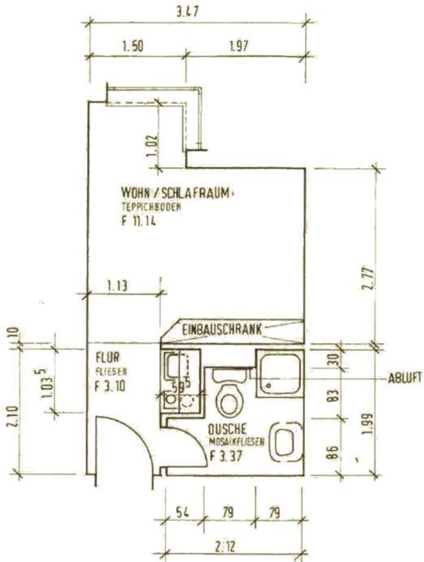
GRUNDRISS APP. 140
