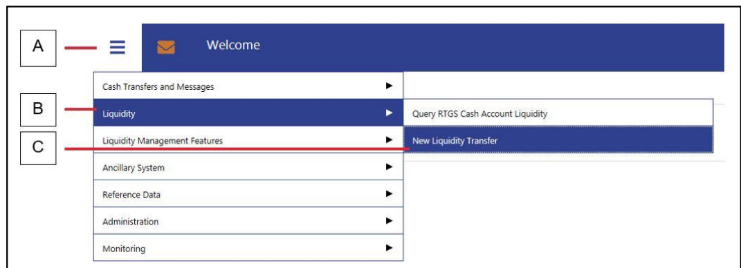
Figure 1 - RTGS Menu
