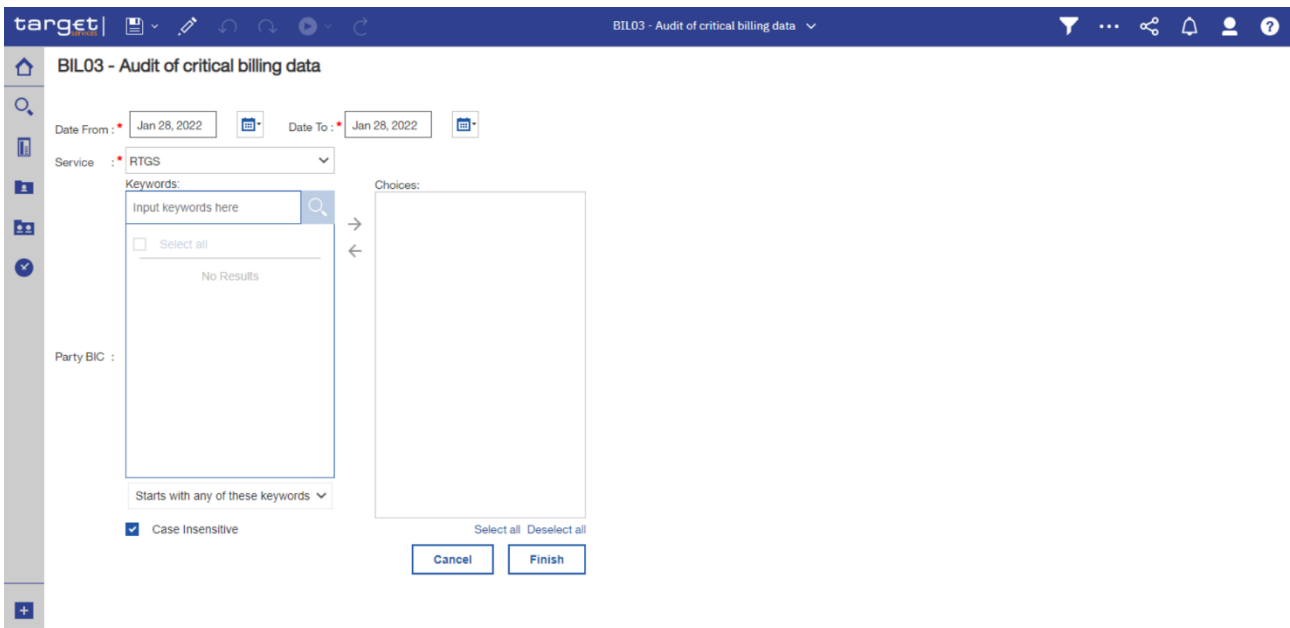
Figure 197 - BIL03 prompt
