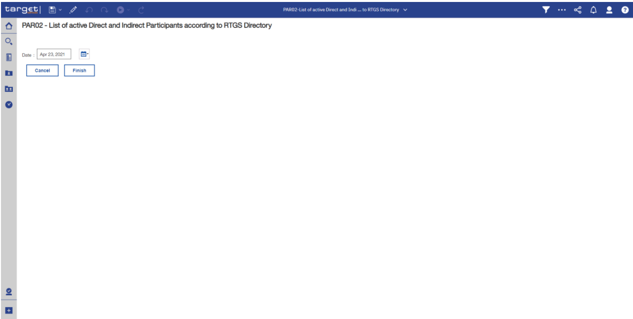
Figure 285 - PAR02 prompt
