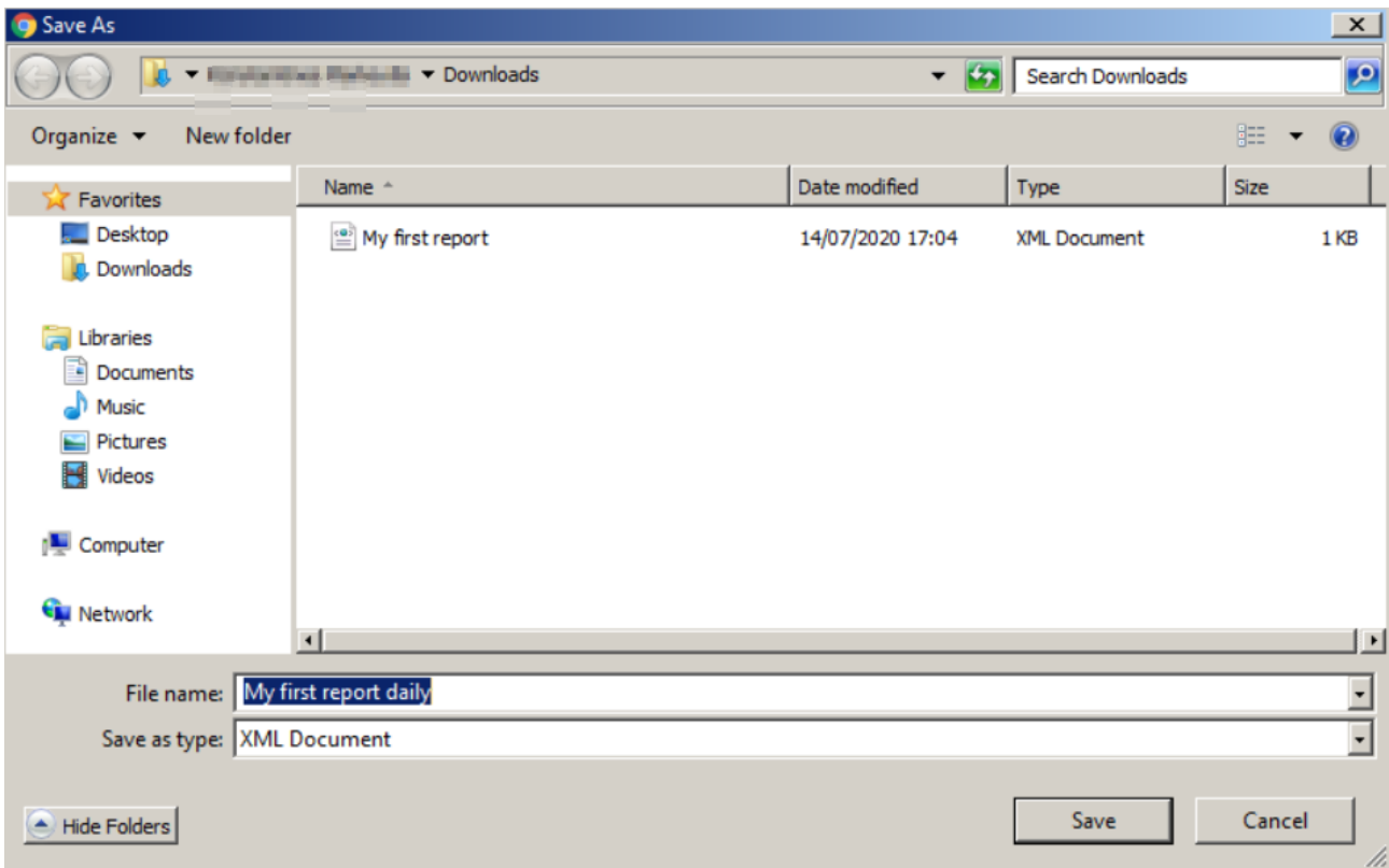
Figure 84 - Save Report
