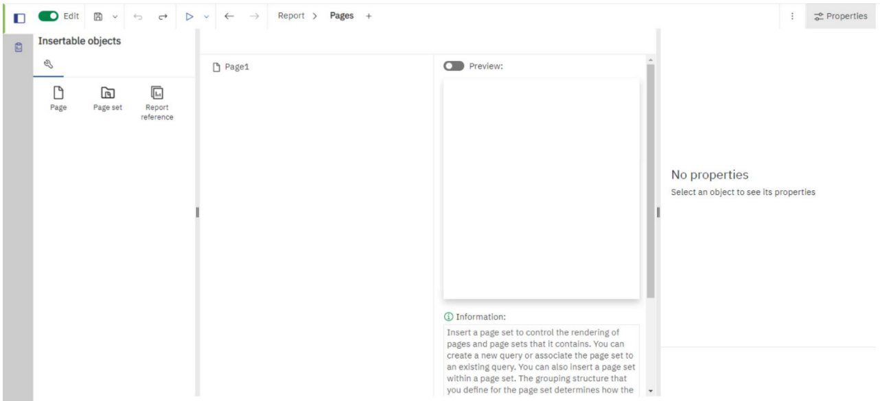
Figure 448 - Pages pane
