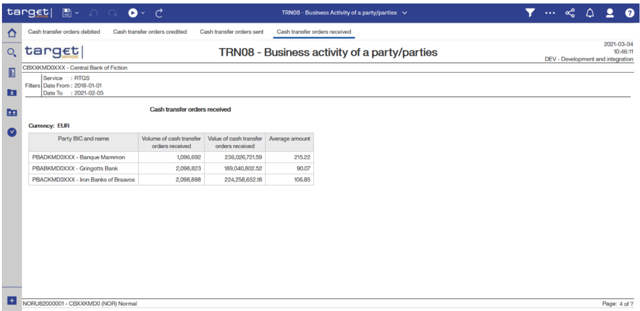
Figure 355 - TRN08 output (4)
