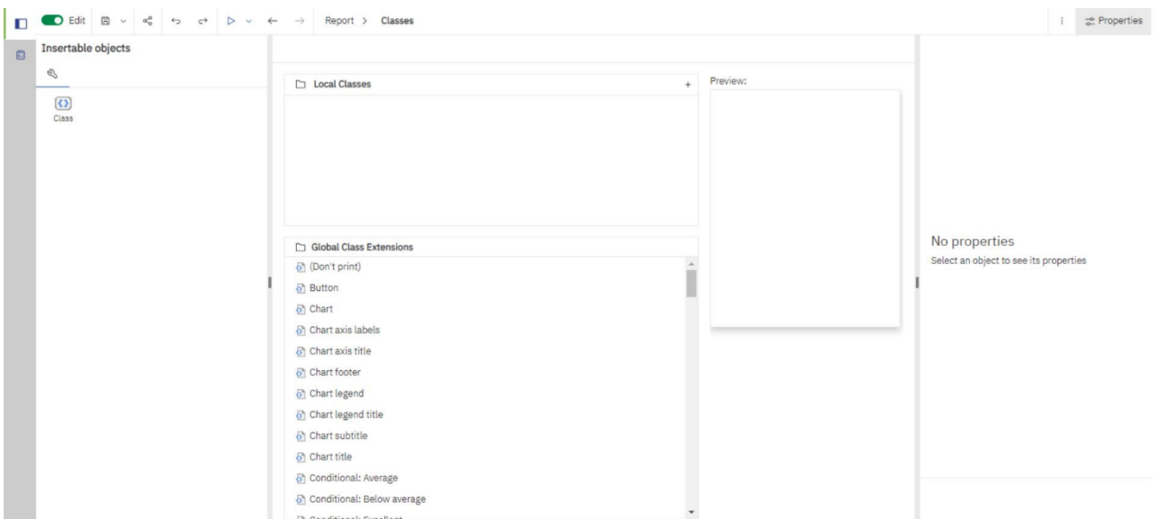
Figure 450 - Classes pane
