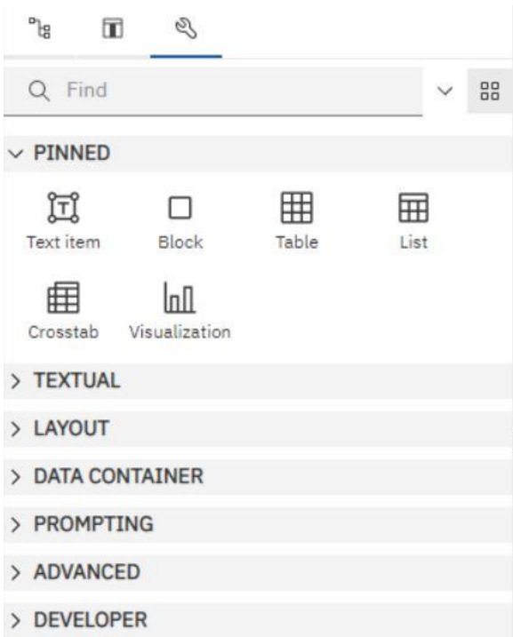
Figure 444 - Toolbox bar
