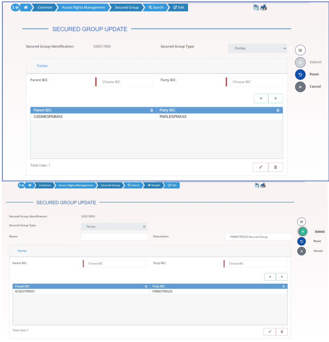
Illustration 84: Secured Group – new/edit screen
