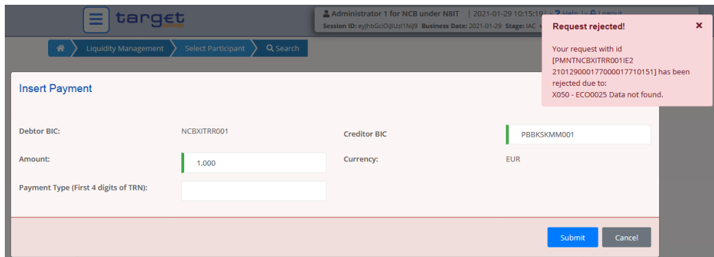
Illustration 10: Error message
