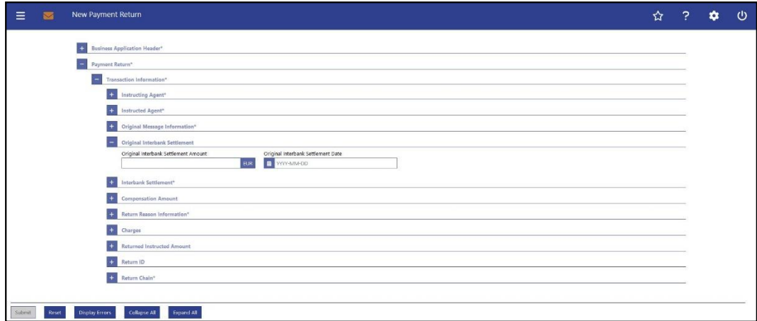
Figure 196 - Payment Return – New Screen – Original Interbank Settlement
