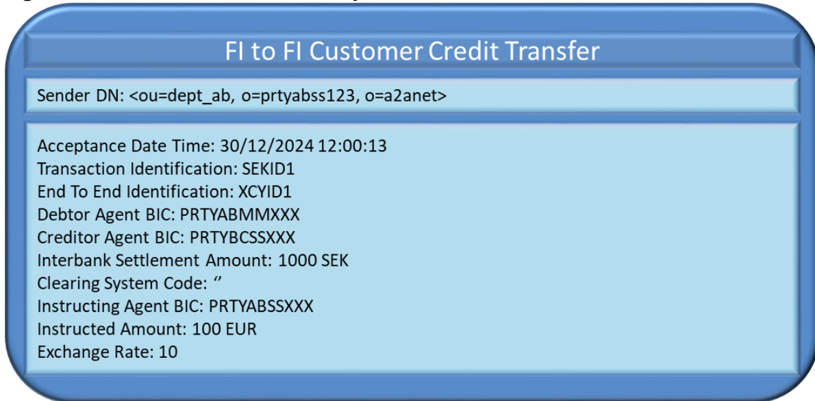
Figure 126 – Successful Instant Payment transaction: FItoFICustomerCreditTransfer
