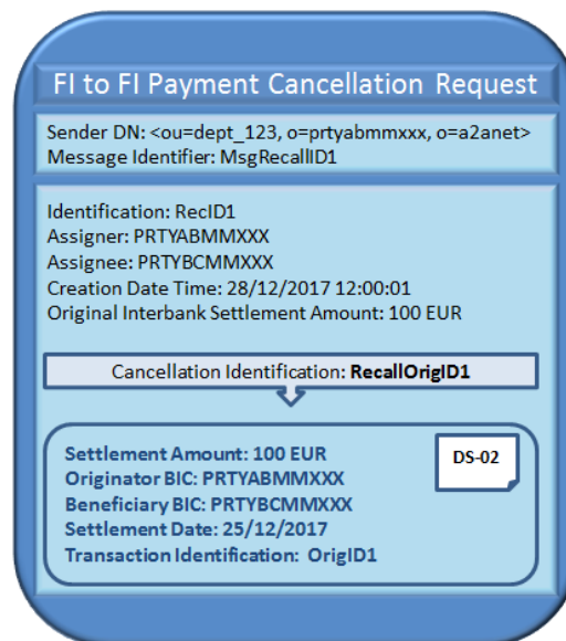
Figure 146 – Recall unsuccessful scenario: Duplicate check failed – FIttoFIPaymentCancellationRequest
