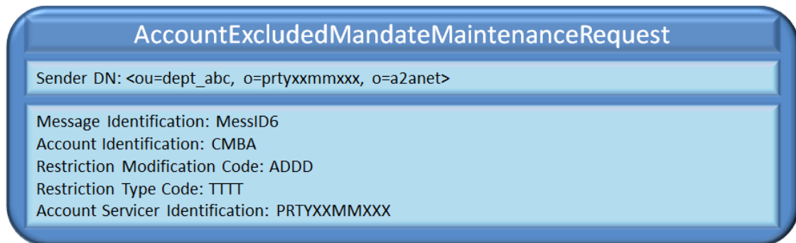
Figure 255 – Unsuccessful block of a CMB: AccountExcludedMandateMaintenanceRequest
