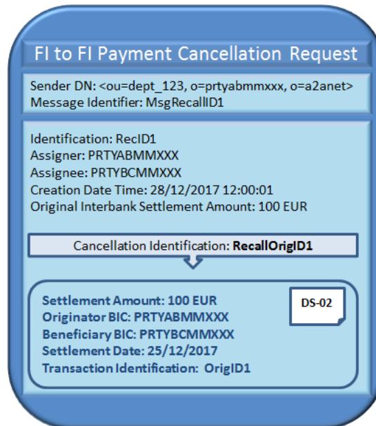
Figure 144 – Recall successful scenario: negative response – FItoFIPaymentCancellationRequest
