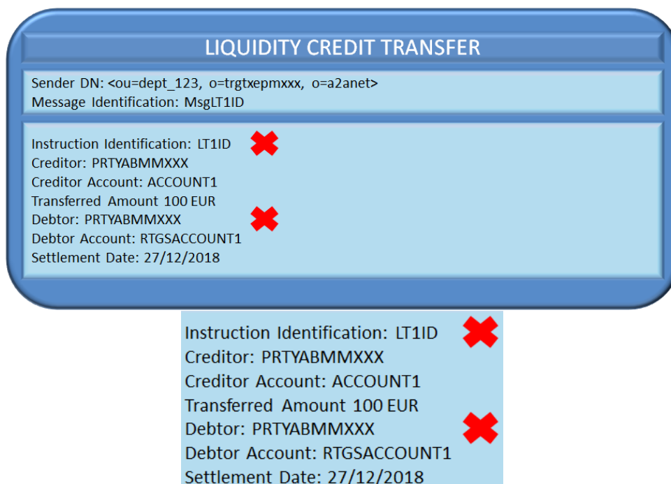
Figure 170 – Unsuccessful Inbound Liquidity Transfer order: duplicate submission
