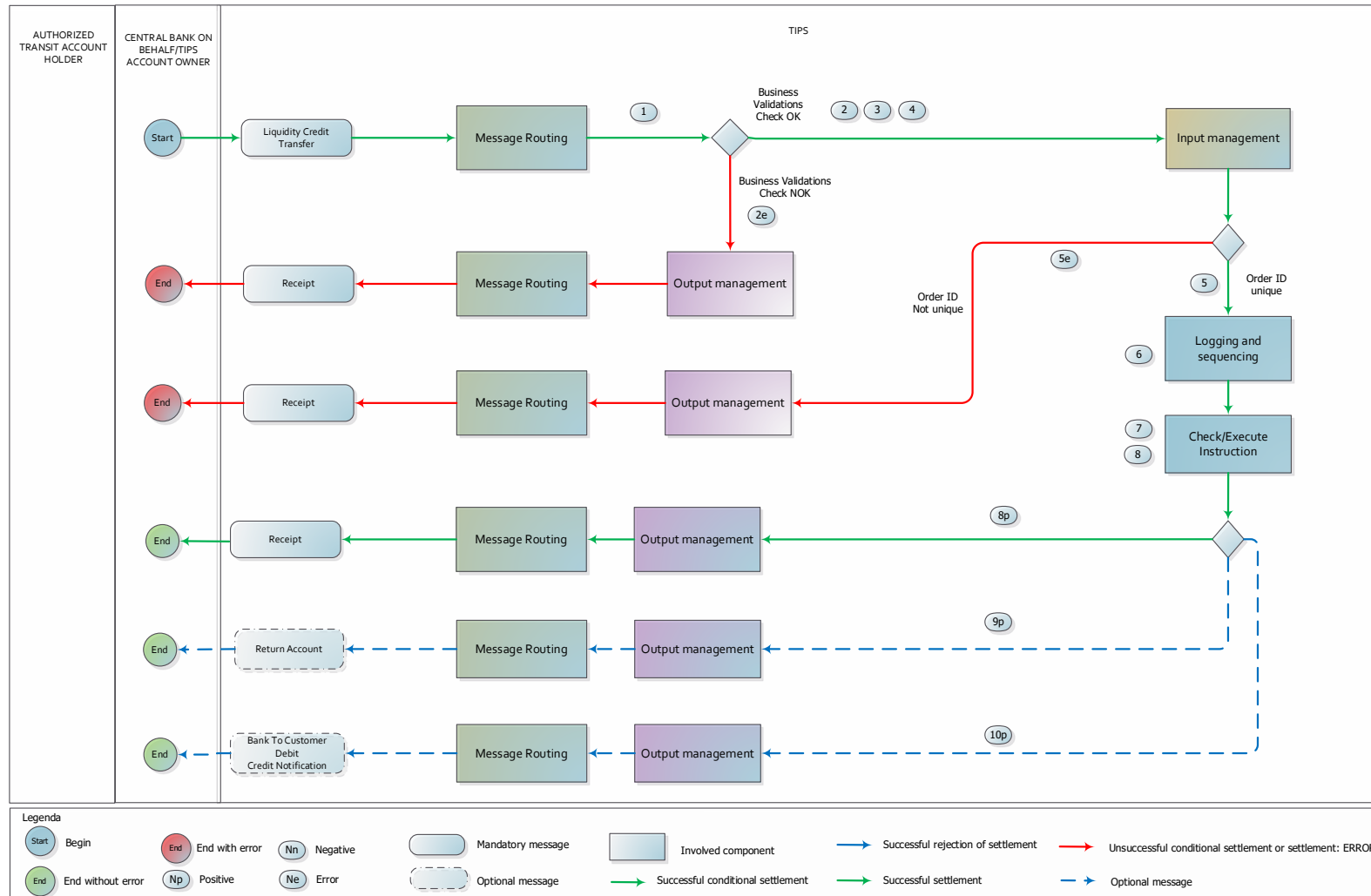
Figure 199 – Internal Contingency Liquidity Transfer flow
