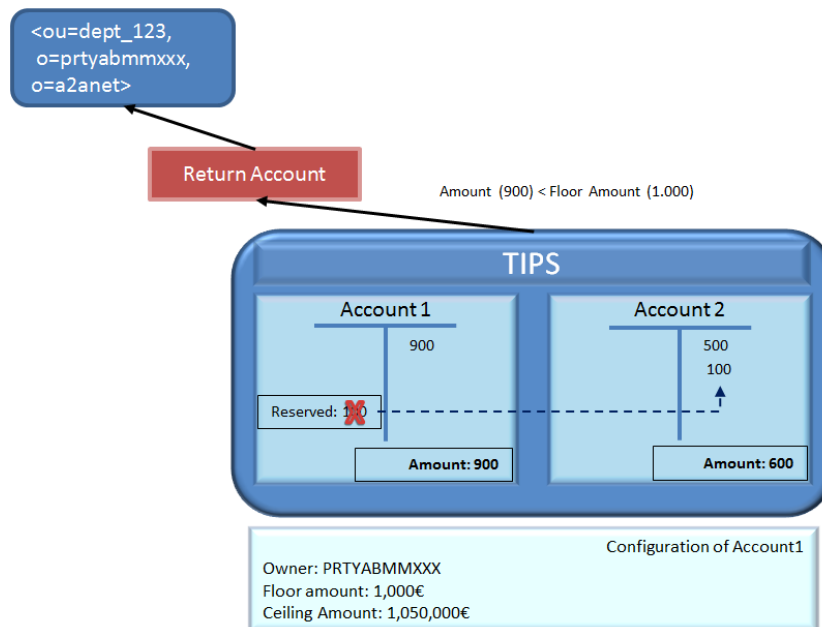
Figure 201 – Floor notification settlement
