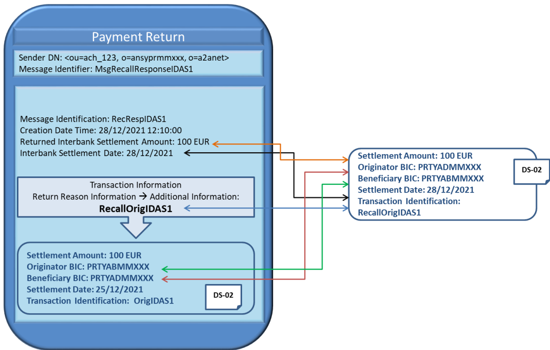
Figure 153 – Recall successful scenario: positive response – Recall Dataset
