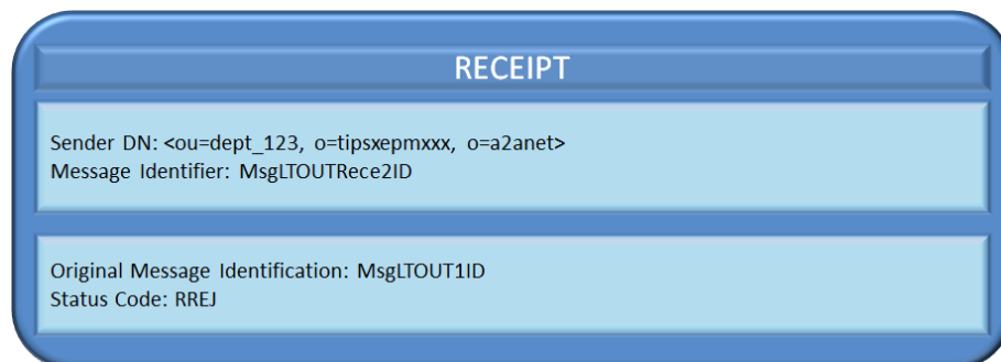
Figure 187 – Outbound Liquidity Transfer order: negative Receipt sent by TIPS
