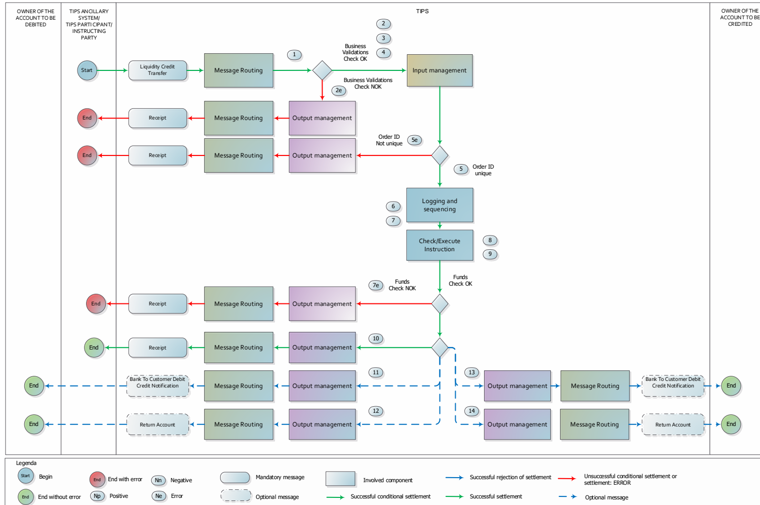
Figure 189 – Intra-service Liquidity Transfer diagram
