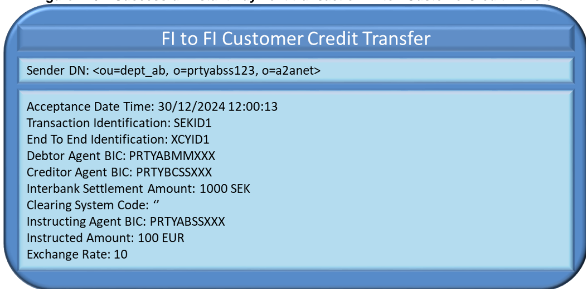
Figure 126 – Successful Instant Payment transaction: FltoFICustomerCreditTransfer
