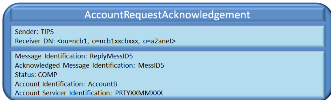
Figure 254 – Successful unblock of an Account: AccountRequestAcknowledgement
