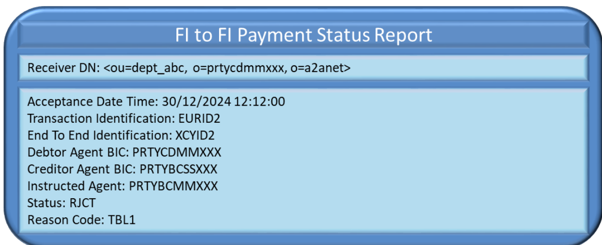
Figure 132 – Blocked account error: FIttoFIPaymentStatusReport
