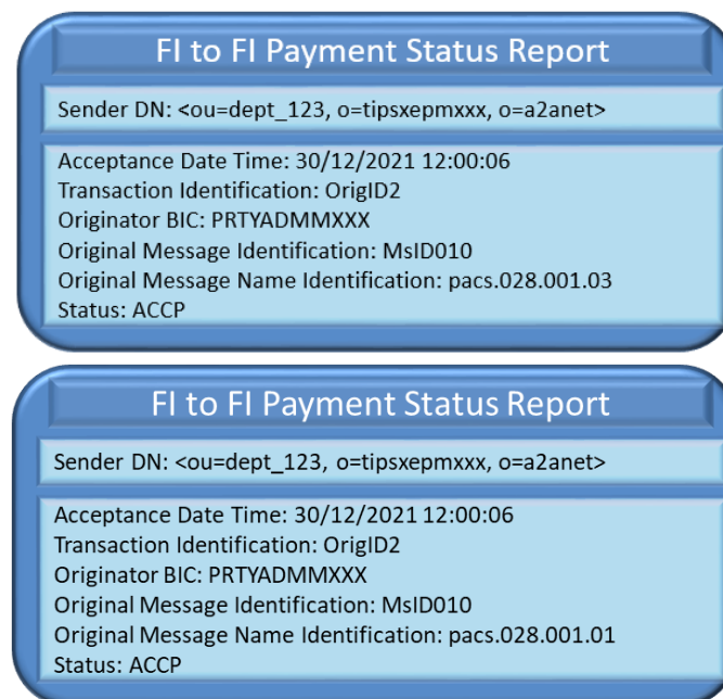
Figure 162 – Successful FIToFIPaymentStatusReport forwarded to an AS
