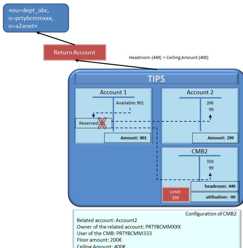
Figure 203 – Ceiling notification settlement
