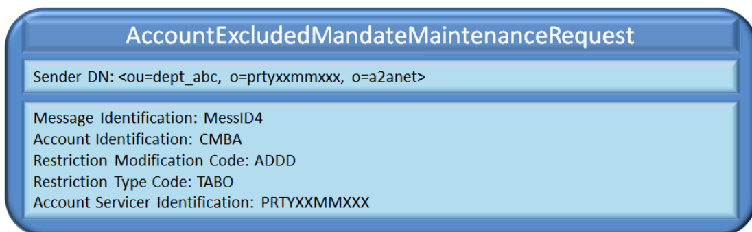
Figure 249 – Successful block of a CMB: AccountExcludedMandateMaintenanceRequest
