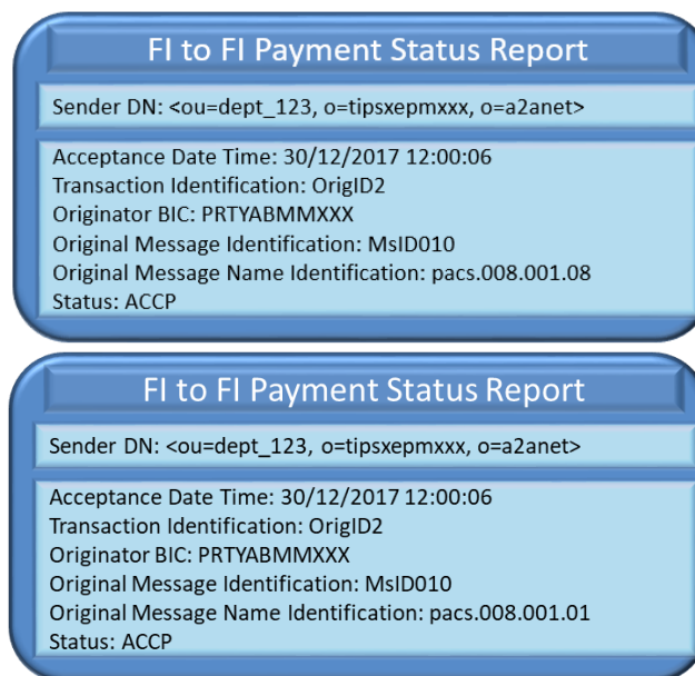
Figure 158 – Successful FIToFIPaymentStatusReport
