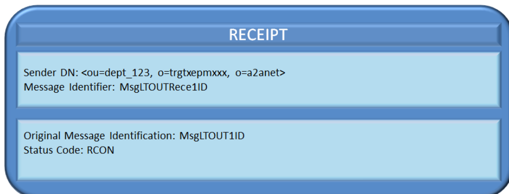
Figure 177 – Successful Outbound Liquidity Transfer order Receipt received by TIPS
