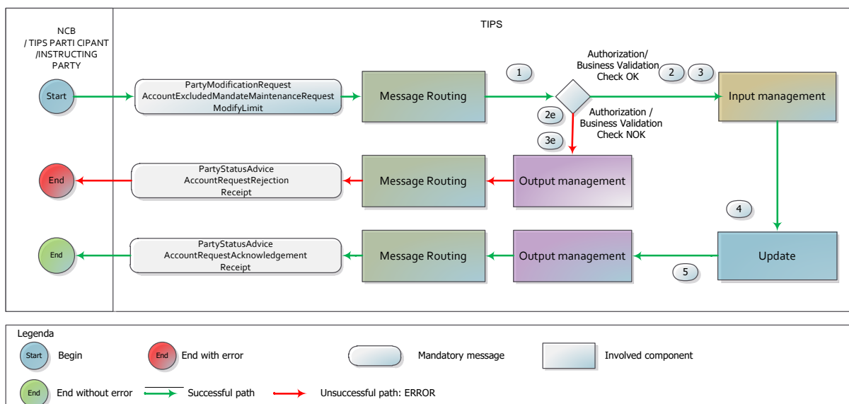
Figure 236 – Reference Data Messages flow
