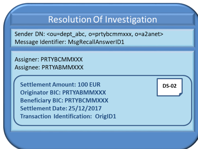
Figure 145 – Recall successful scenario: negative response – ResolutionOfInvestigation
