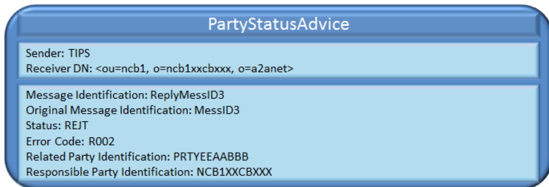
Figure 248 – Successful block of a TIPS Participant: PartyStatusAdvice
