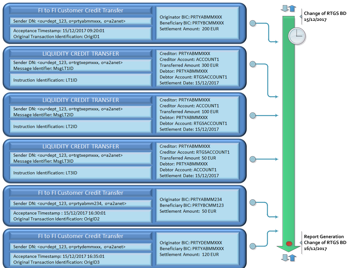
Figure 229 – Statement of Accounts example: list of transactions (full mode)
