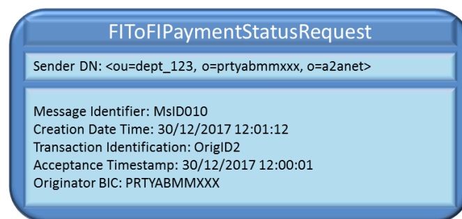
Figure 157 – Successful FIToFIPaymentStatusRequest
