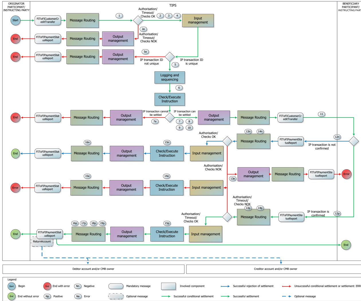
Figure 20 – Instant Payment transaction flow
