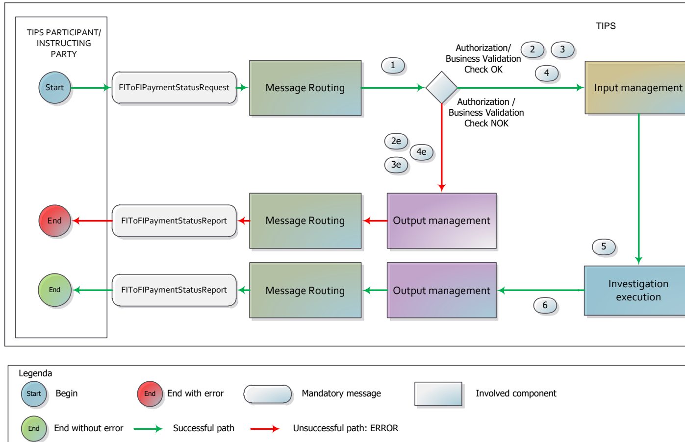
Figure 155 – Investigation Flow
