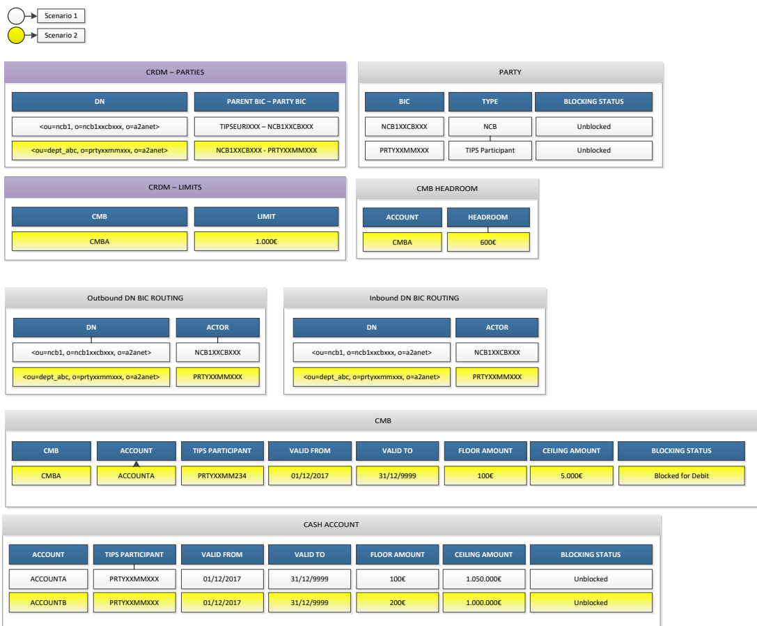
Figure 237 – Reference Data Management examples: data constellation
