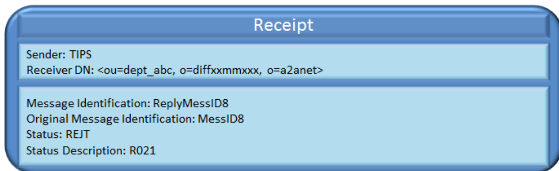
Figure 261 – Unsuccessful decrease of a CMB Limit: Receipt
