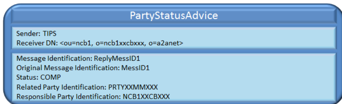
Figure 240 – Successful block of a TIPS Participant: PartyStatusAdvice
