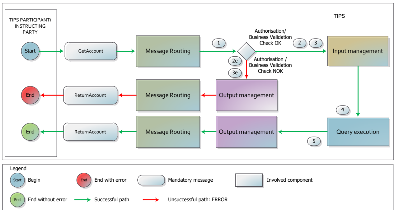
Figure 205 – Account Balance Status query flow
