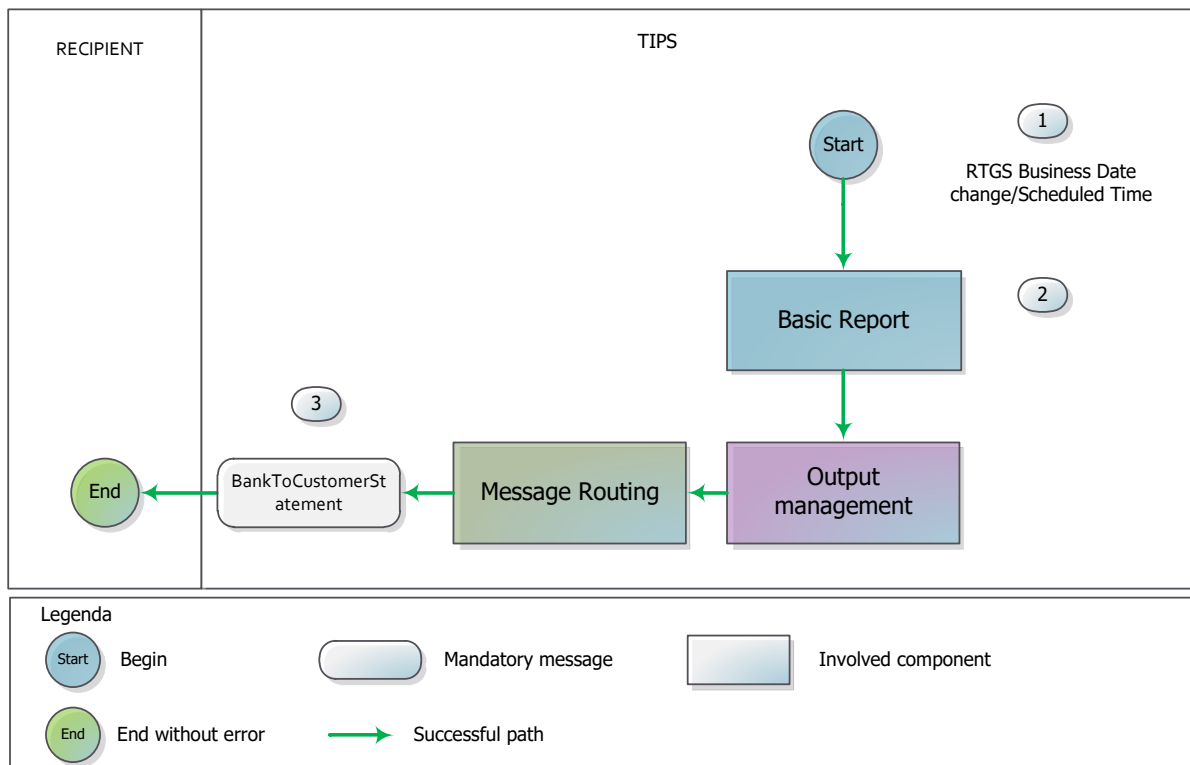
Figure 225 – Statement of Accounts flow
