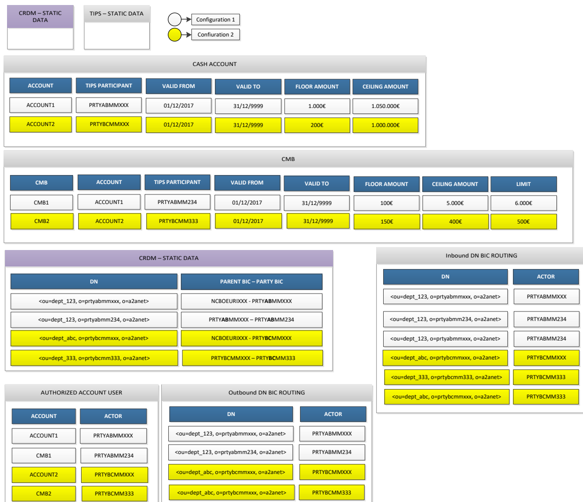
Figure 156 – Transaction status investigation examples: data constellation
