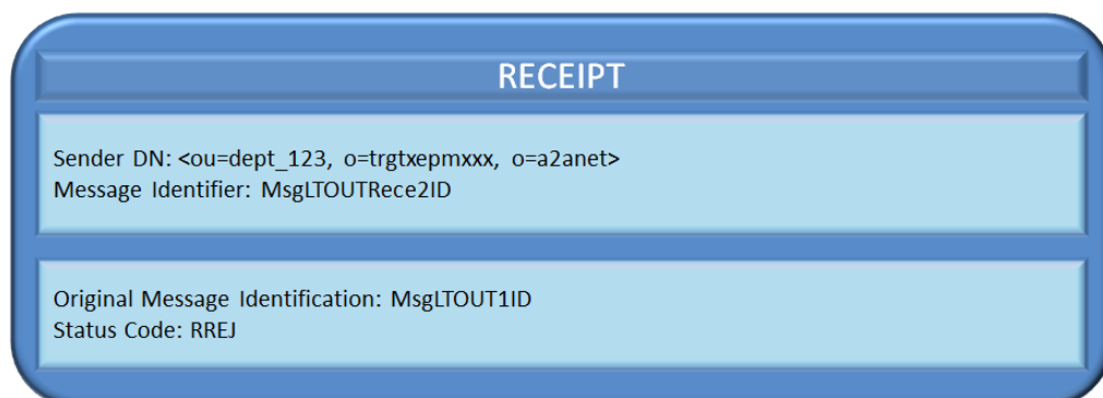
Figure 185 – Outbound Liquidity Transfer order: negative Receipt sent by the RTGS System
