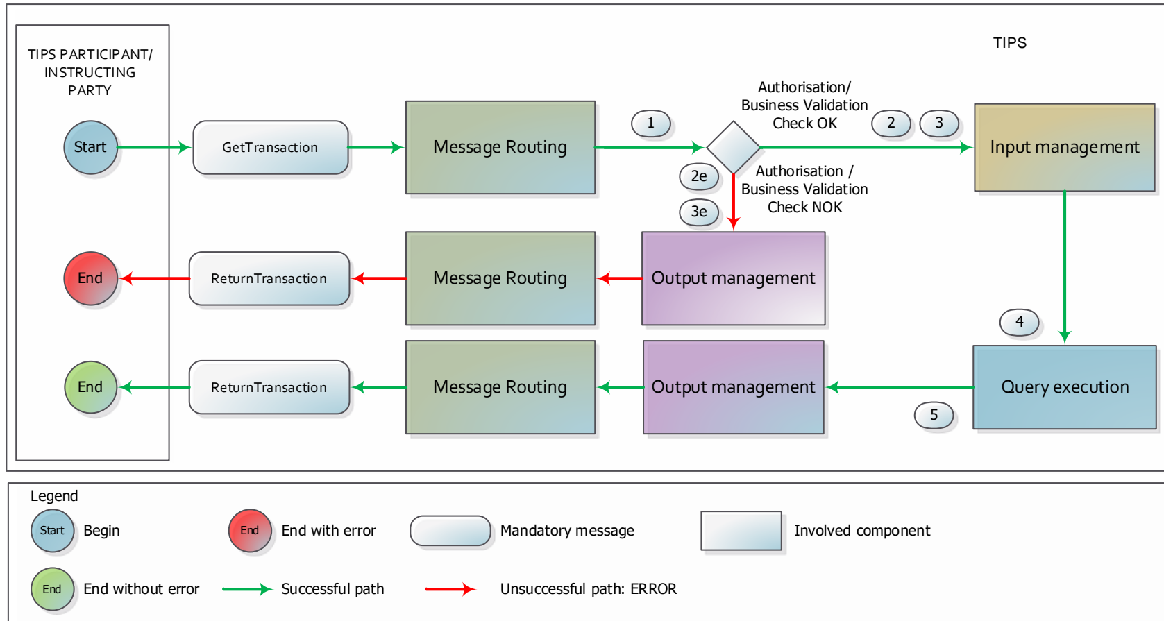
Figure 206 – Payment transaction status query flow
