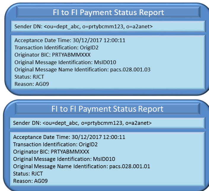
Figure 160 – Unsuccessful FIToFIPaymentStatusReport
