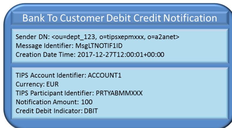
Figure 179 – Successful Outbound Liquidity Transfer order debit notification
