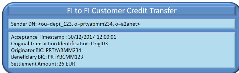
Figure 27 – Successful Instant Payment transaction: FltoFICustomerCreditTransfer
