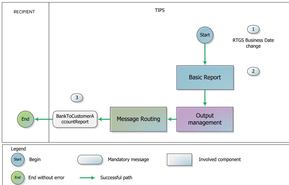
Figure 220 – Statement of Account Turnover flow
