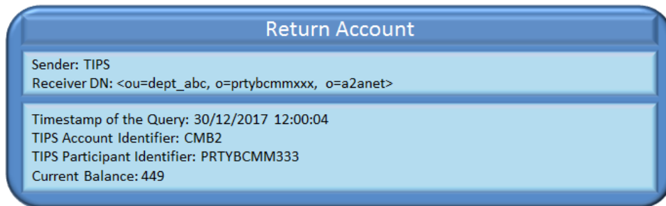
Figure 204 – Ceiling notification ReturnAccount
