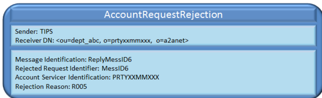
Figure 256 – Unsuccessful block of a CMB: AccountRequestRejection
