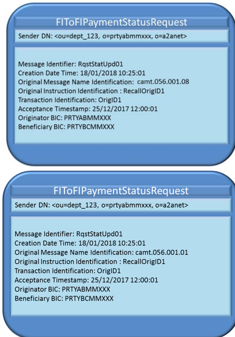
Figure 150 – Successful request for Status Update on a Recall
