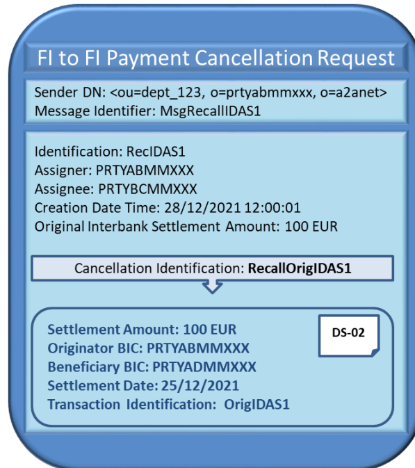
Figure 151 – Recall successful scenario: positive response – FItoFIPaymentCancellationRequest
