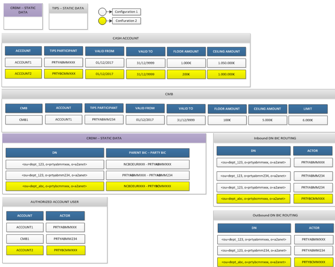
Figure 207 – Queries examples: data constellation
