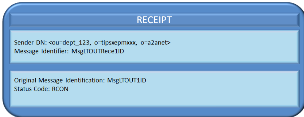
Figure 178 – Successful Outbound Liquidity Transfer order Receipt sent by TIPS
