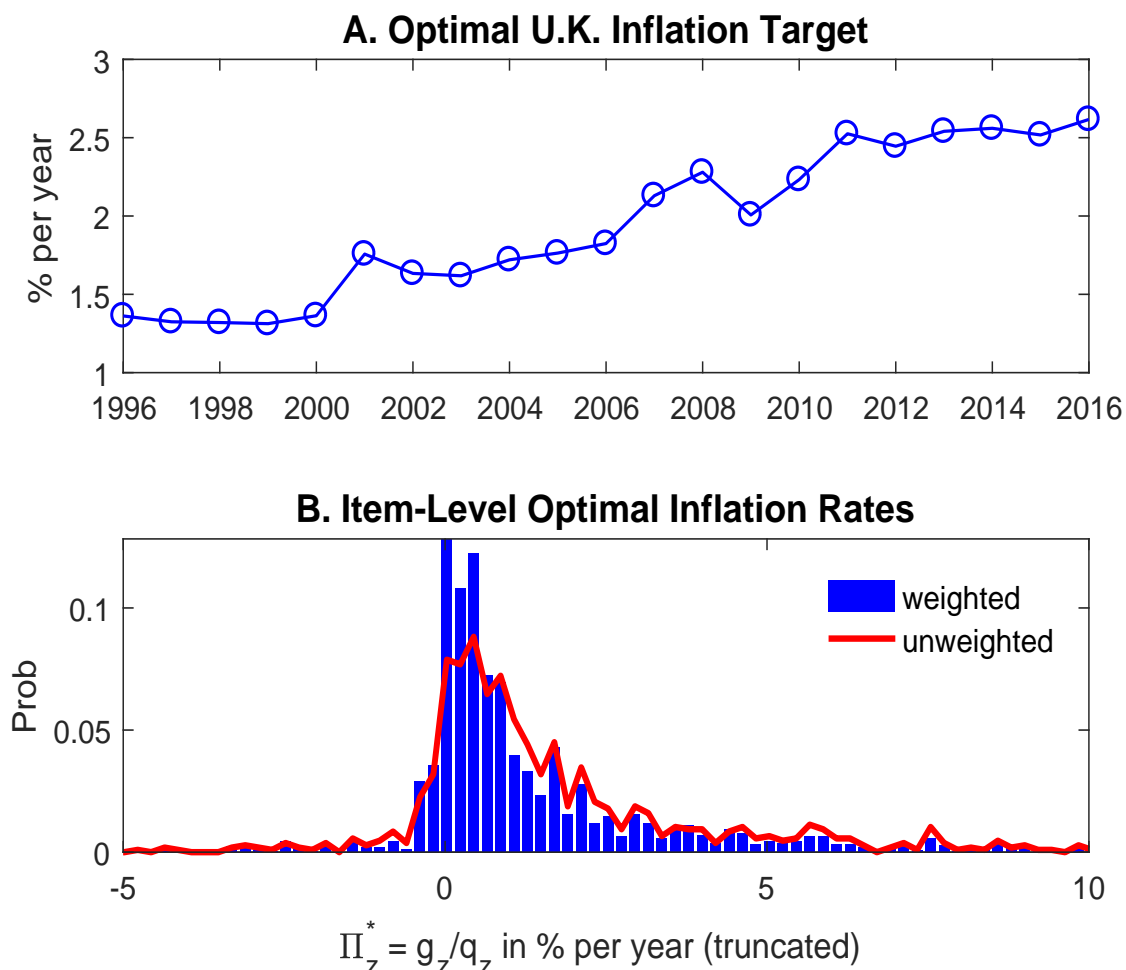
Figure 5: Optimal U.K. Target - Baseline Results
