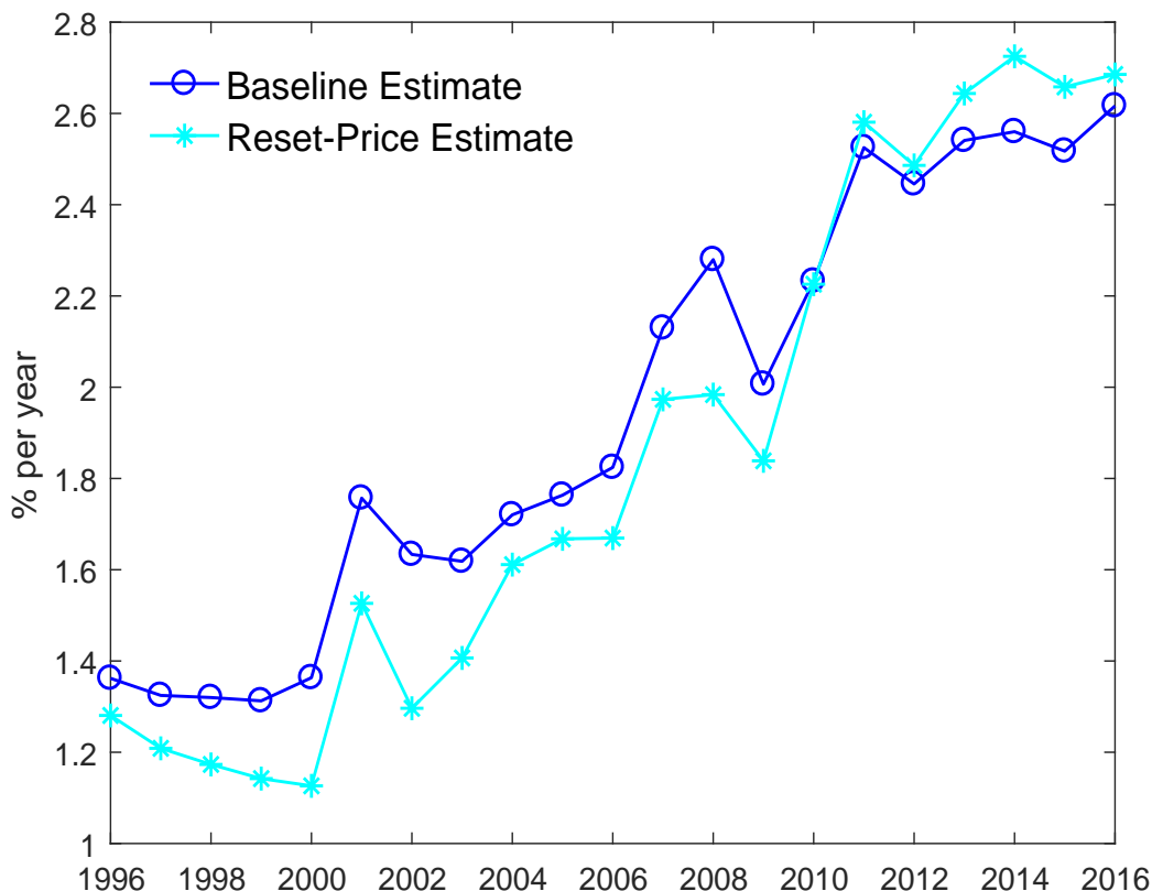
Figure 9: Optimal inflation target: baseline versus reset price based estimation
