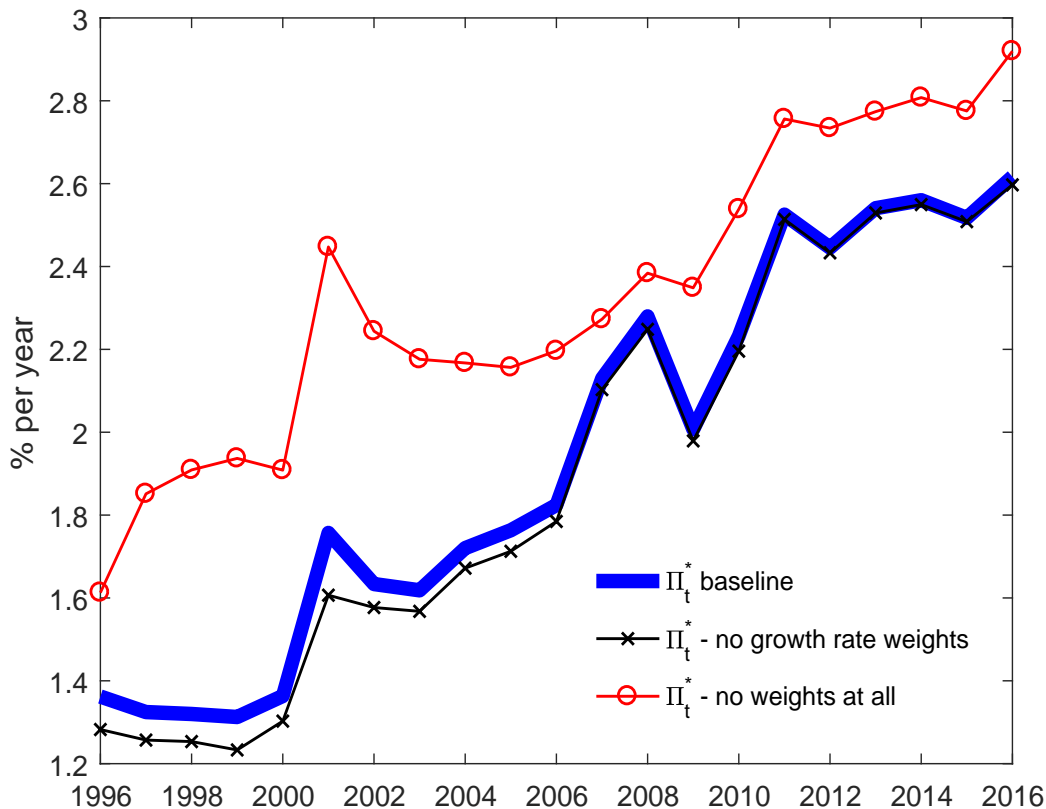
Figure 8: Relevance of the weighting schemes for the estimated optimal inflation target
