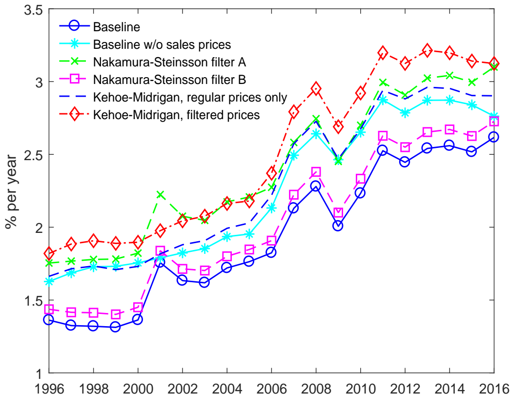
Figure 10: Optimal inflation target for alternative treatments of sales prices
