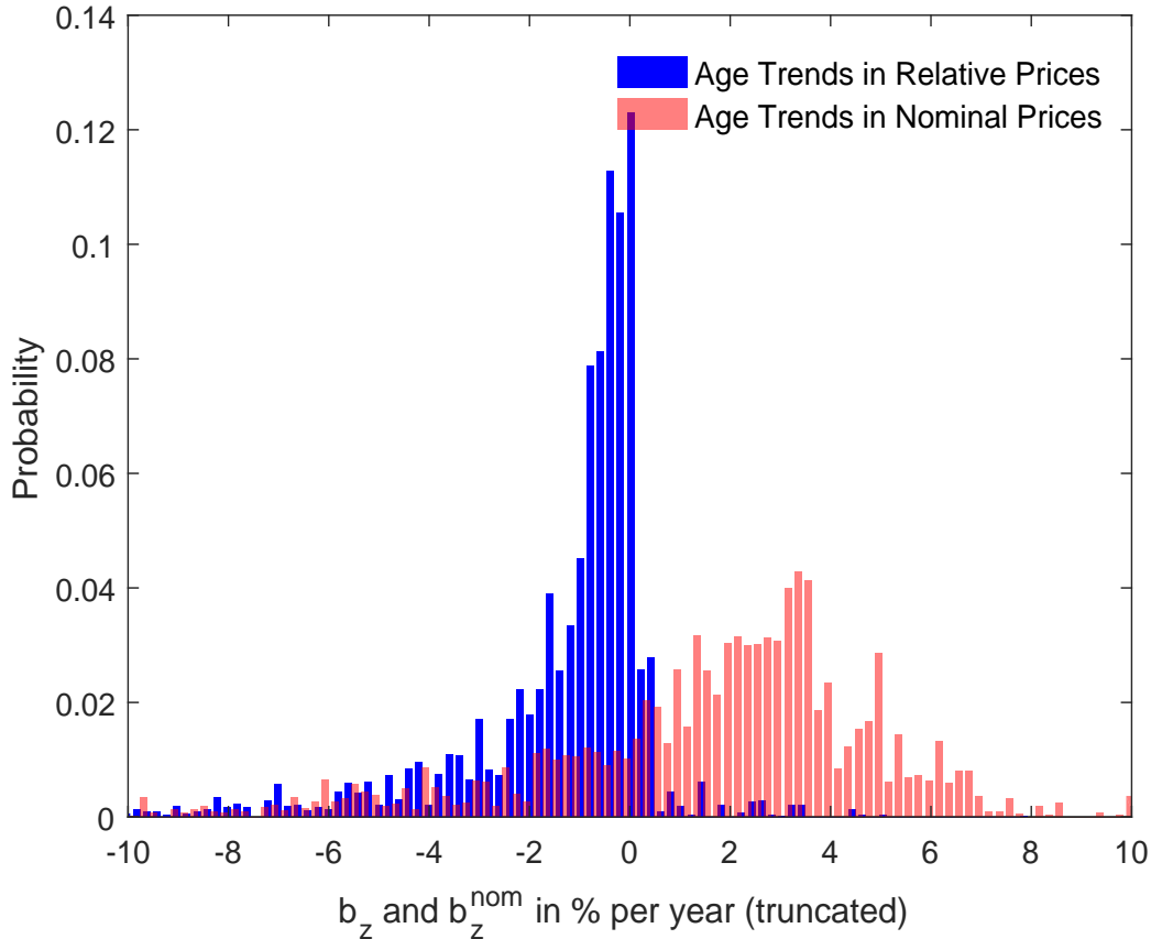
Figure 3: Distribution of Age Trend Coefficients from Regression 1) with Relative Prices ( \ln \tilde{P}_{jzt}/P_{zt} ) and Nominal Prices ( \ln \tilde{P}_{jzt} ) as l.h.s. Variable.
