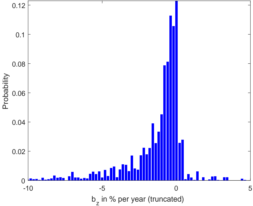
Figure 2: Distribution of Estimated Slope Coefficients Across Items from Equation (1)
