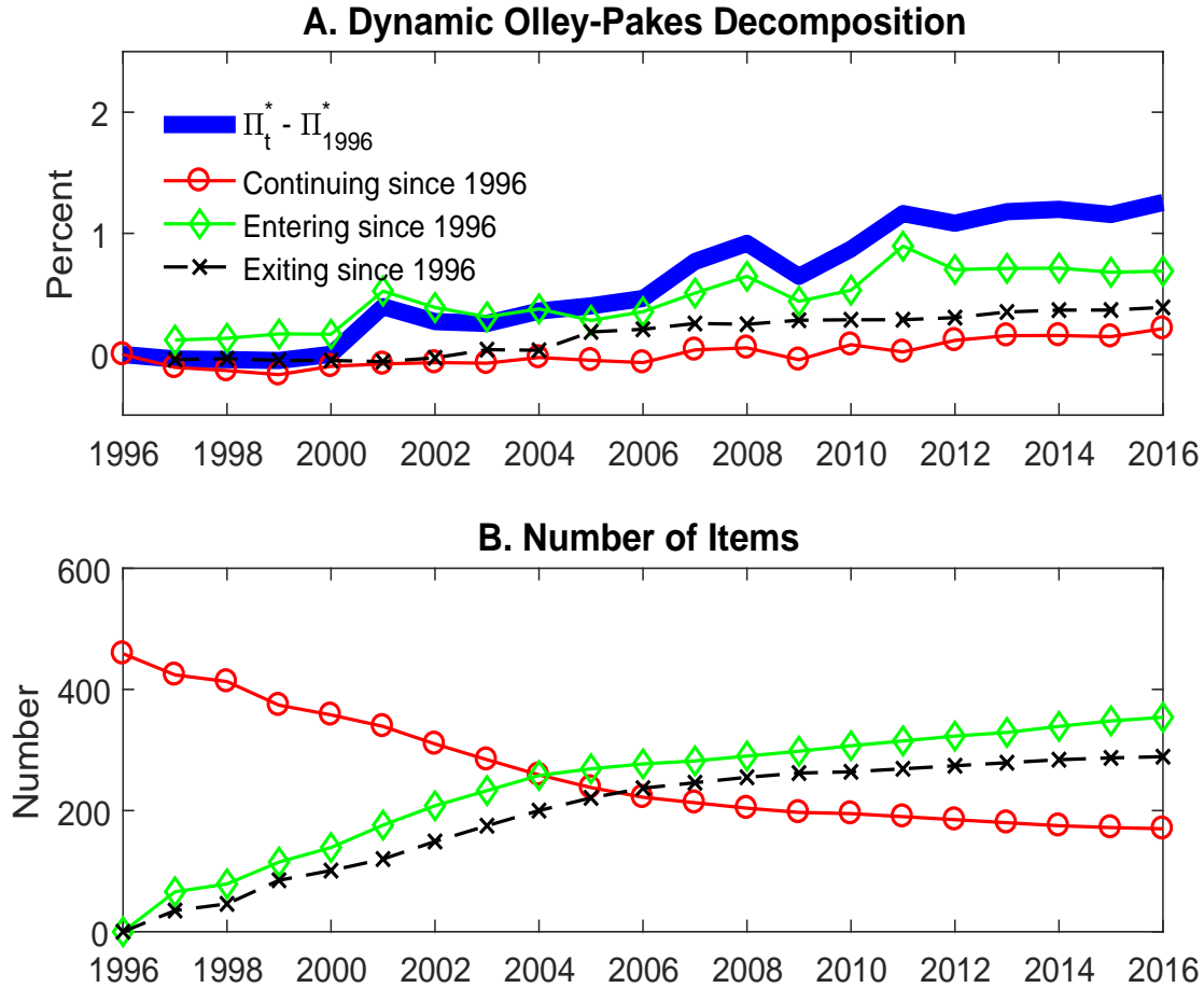
Figure 6: Decomposing the upward trend in the optimal inflation target
