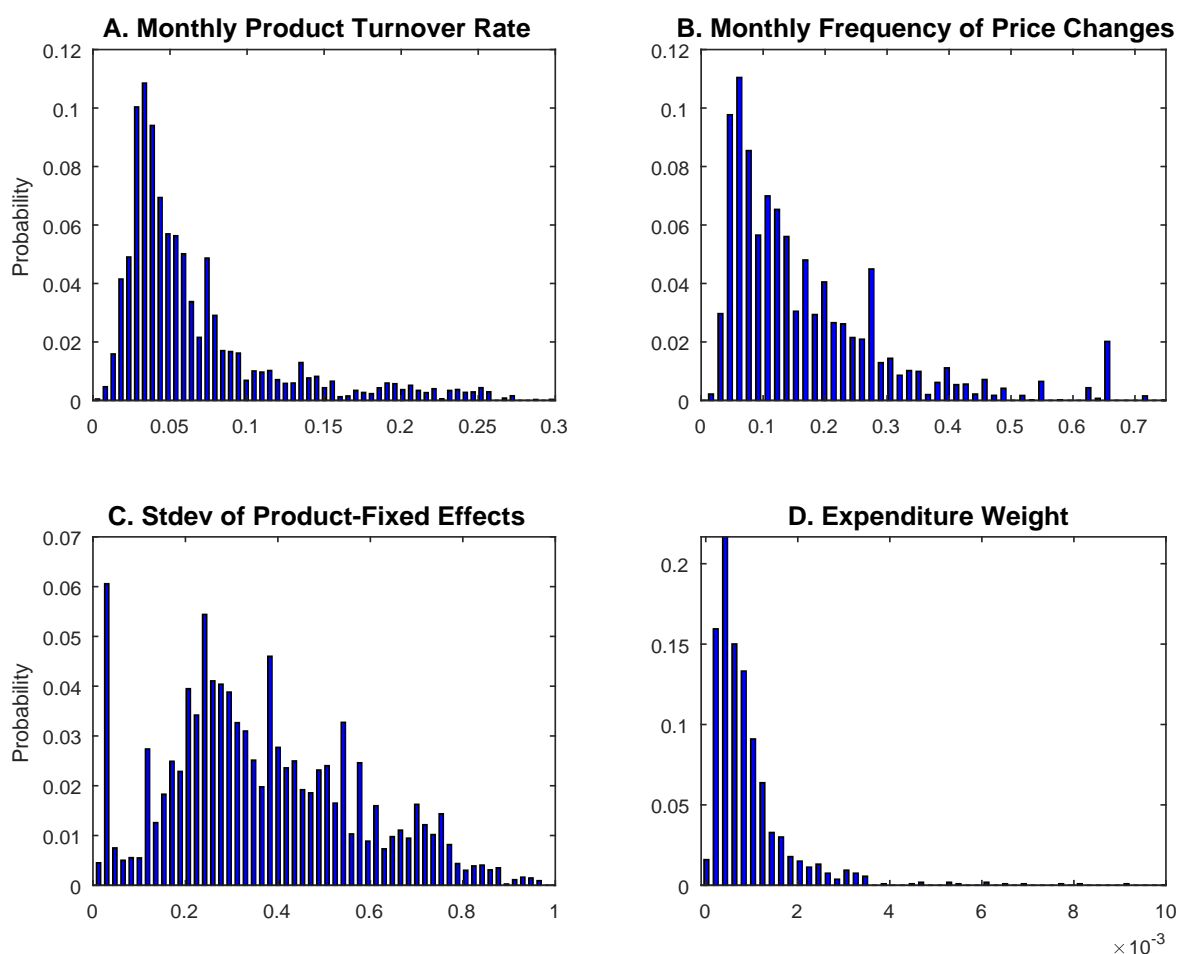
Figure 4: Distribution of Various Variables across Items
