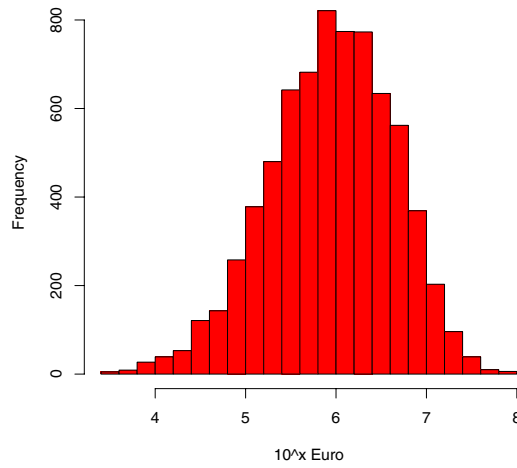
Figure 2: Histogram of the exposure sizes in the credit portfolio logarithmic scale.
