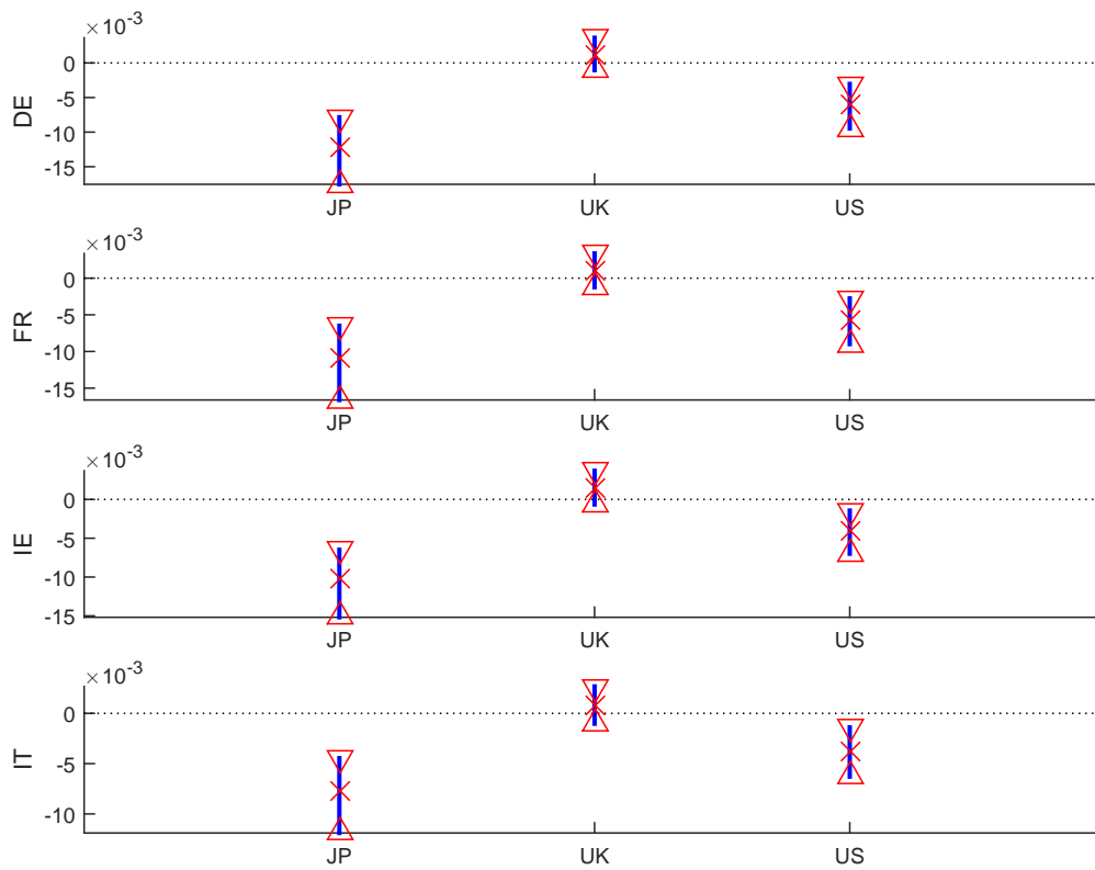
Figure 7: Effects of general risk shocks on the Euro
