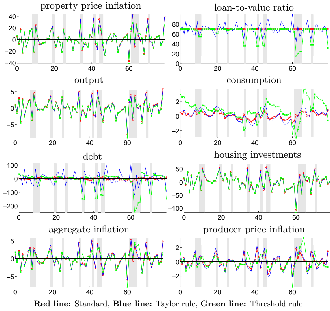
Figure 3. Simulations of the Model for \sigma_{d,s} = 2.2
