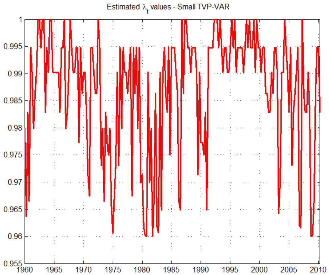
Figure 2: Values of the time-varying forgetting factor \lambda_t for the small TVP-VAR, estimated according to equation (6).
