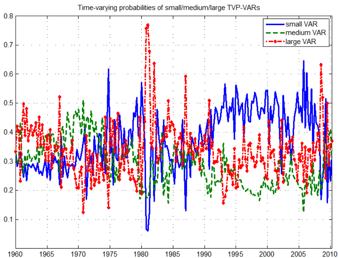
Figure 3: Estimated Dynamic Dimension Selection probabilities of the small, medium and large TVP-VARs.
