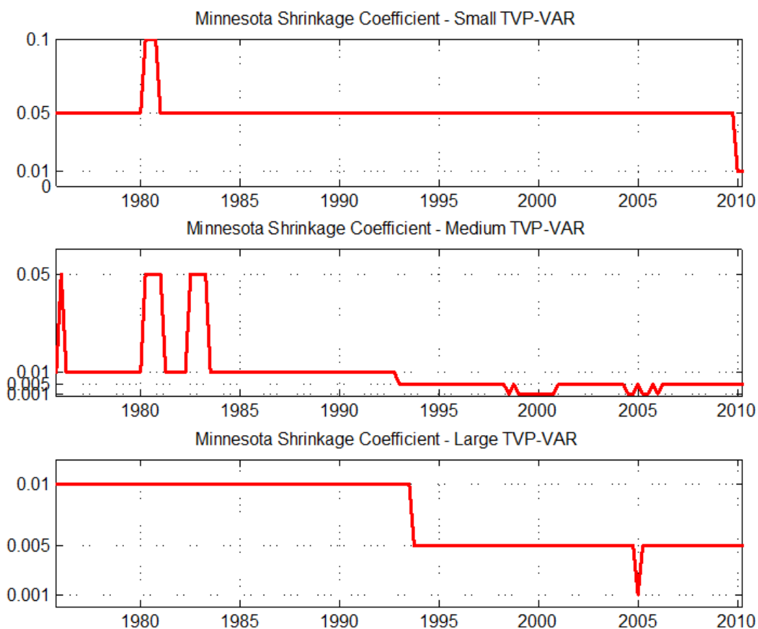
Figure 1: Values of shrinkage coefficients \gamma , estimated for each time period and for each VAR size.
