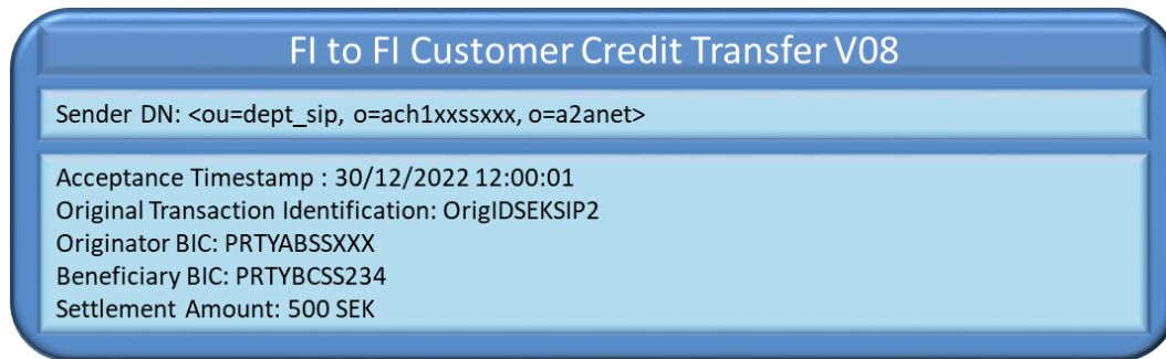
Figure 109 – Successful Instant Payment in non-Euro currency with SIP: FIToFICustomerCreditTransfer
