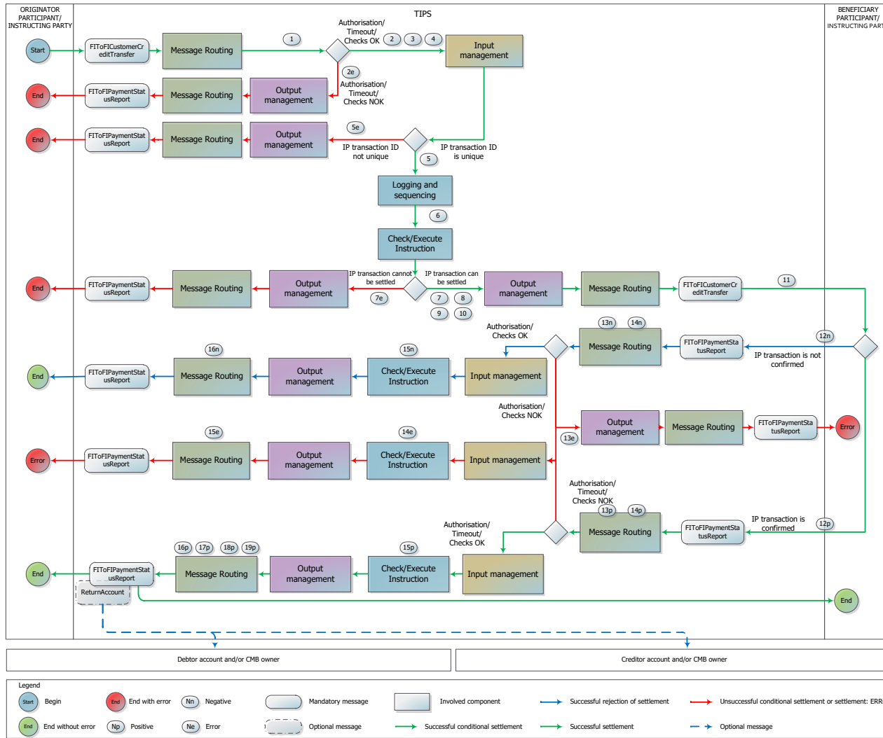
Figure 19 – Instant Payment transaction flow
